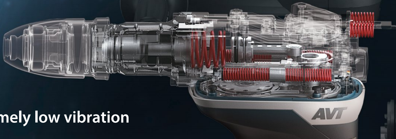
40mm Rotary Hammer HR4013C
