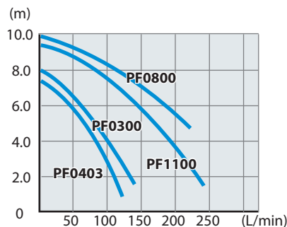
Total Head & Pumping Capacity
